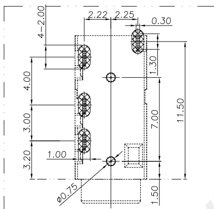
RECOMMENDED P.C.B TOP VIEW
